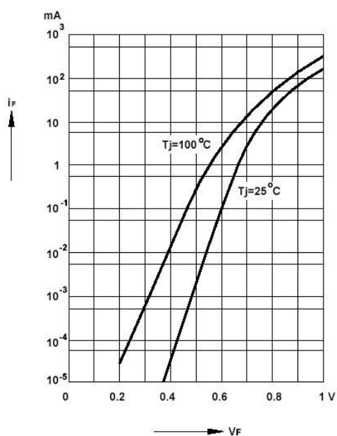
Forward characteristics
